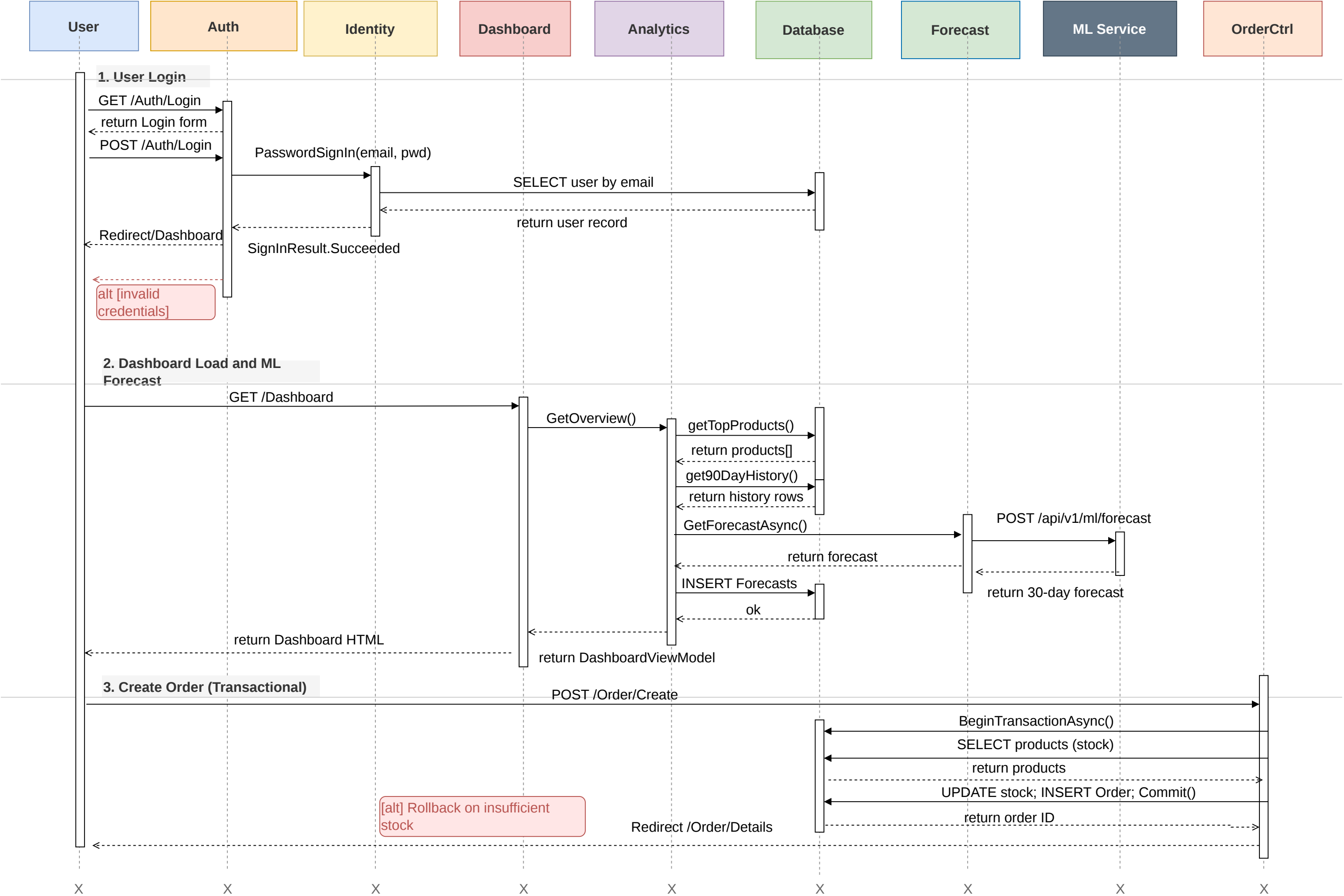
Sequence Diagram: SellWise AI Sales Analytics System
